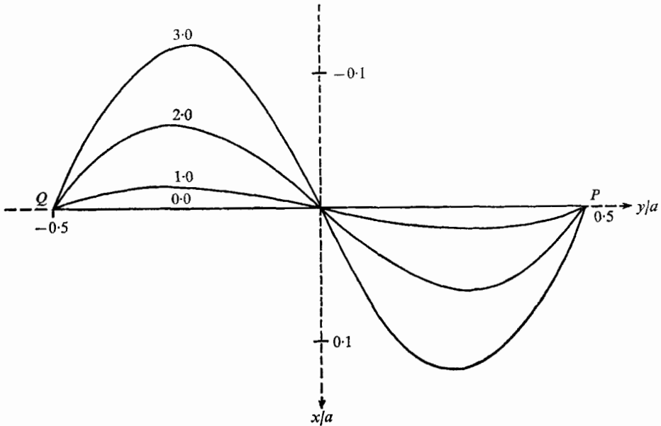
FIGURE 2. The projection of the locus of the centres of rotation on the x, y plane for various values of kh .
